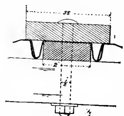
Fig. 2387. Section through Ridge-pole.
